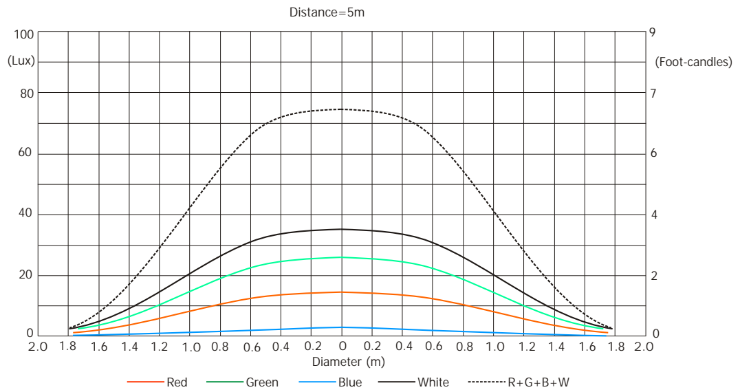
Illuminance distribution in Y-axis
