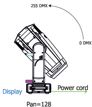
Tilt = 0 DMX
