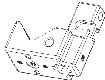
⑩ Lower-casting
