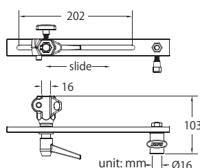
Safety wire quipped on the column to avoid clamp unexpected drop-off.
