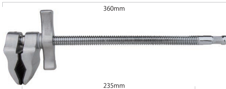
KCP-607 Super Viser Clamp End Jaw 9"(23.5cm)
