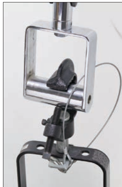
Stirrup head
